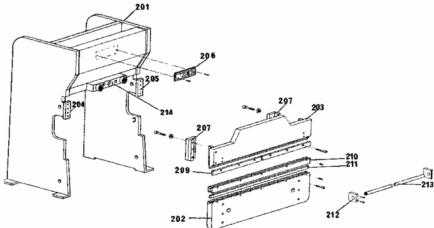
FIGURE 1 — FRAME ASSEMBLY
