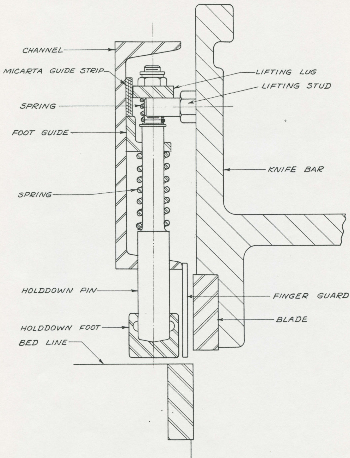
LAYOUT OF TYPICAL HOLDDOWN ASSEMBLY FOR MACHINES THROUGH 1010-RT
