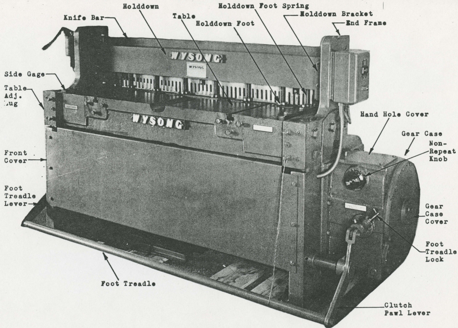
FRONT VIEW
